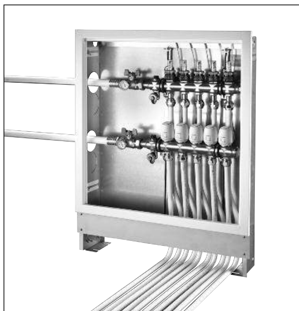
Stainless steel distributor/collector, item no. 14043
